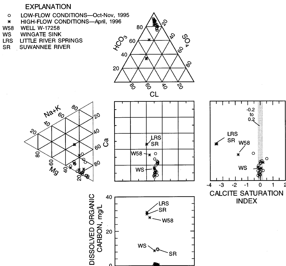
Figure 5 Durov plot showing major-ion composition, dissolved organic carbon, and calcite saturation index of groundwater, river water, and spring water
